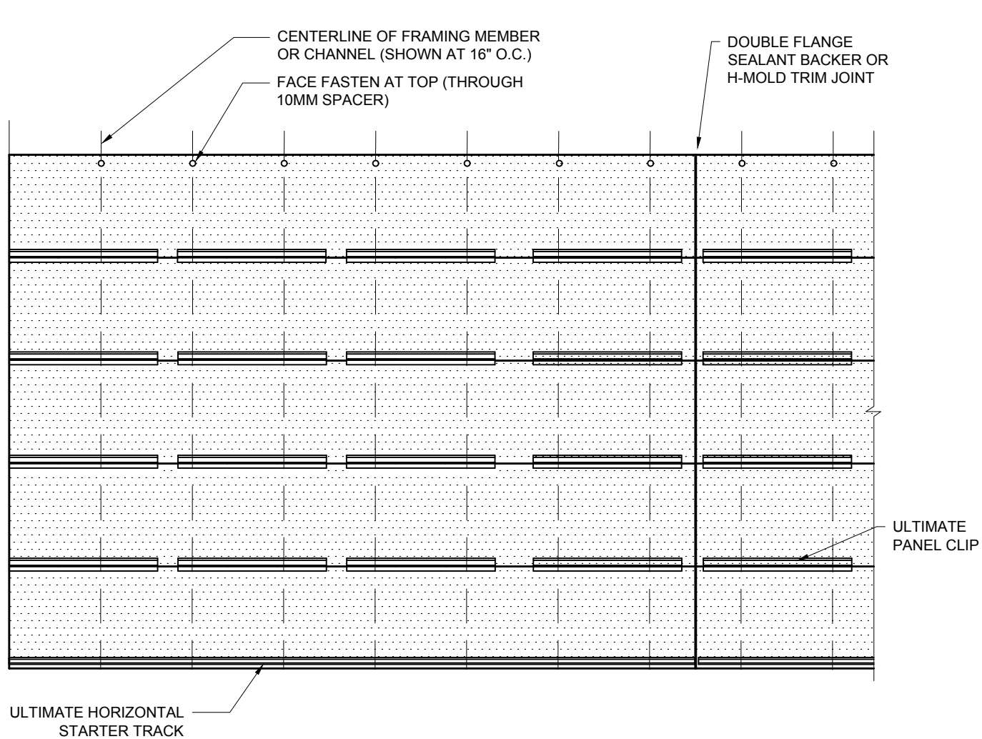
NICHIHA - CLIP PLACEMENT - AWP3030 - STACKED PANEL LAYOUT SCALE: 1/2" = 1'-0"
