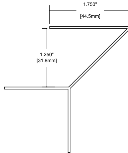
CORNER KEY for 21mm AWP
