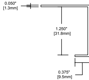
J-MOLD for 21mm AWP
