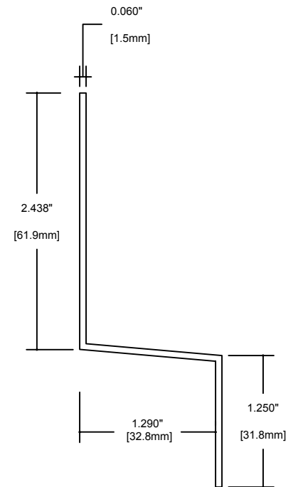
COMPRESSION JOINT FLASHING for 21mm AWP
