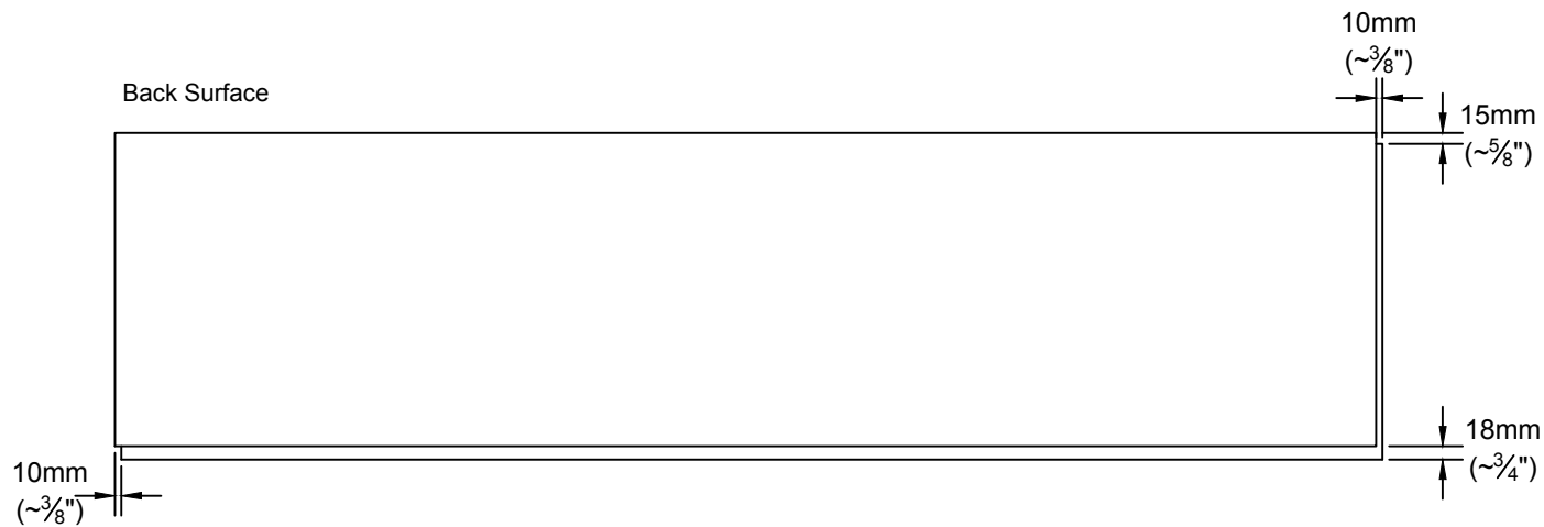
NICHIHA - CORBOSA - PANEL DETAIL SCALE: 1" = 1'-0"
