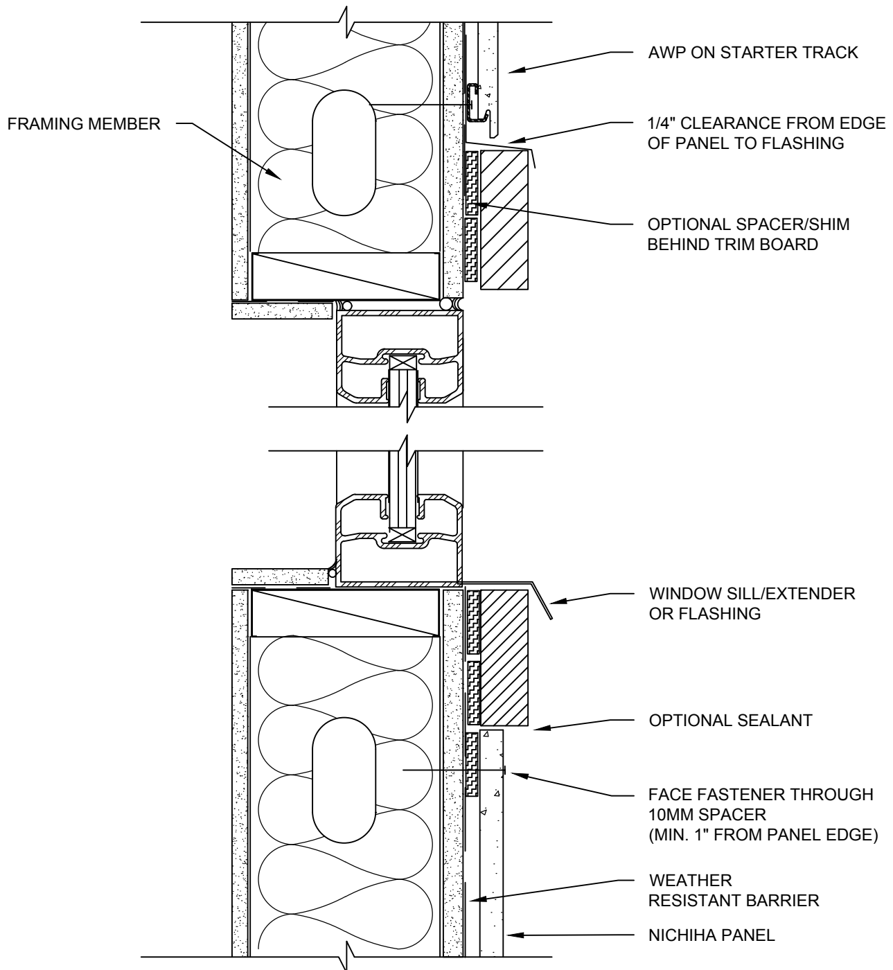
NICHHA - AWP - HORIZONTAL - STUD WALL - STOREFRONT WINDOW - HEADER & SILL WITH TRIM BOARD
