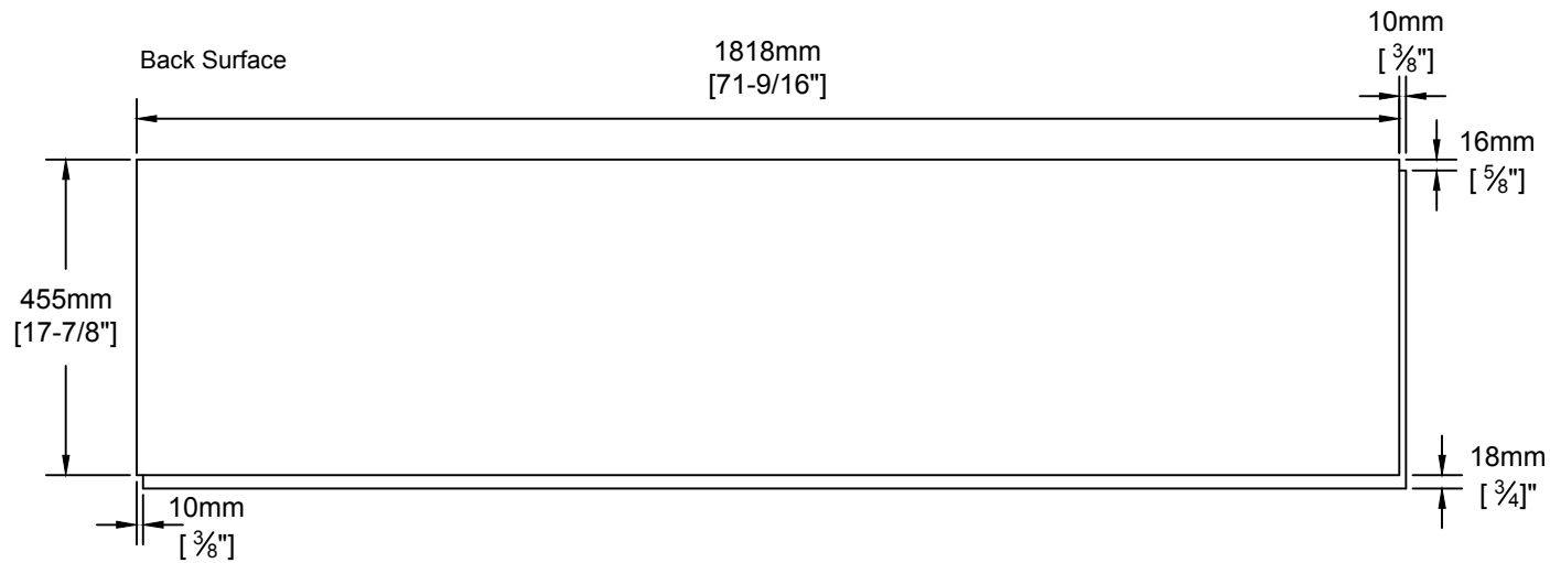
NICHIHA - MODERN BRICK PANEL DETAIL SCALE: 1" = 1'-0"
