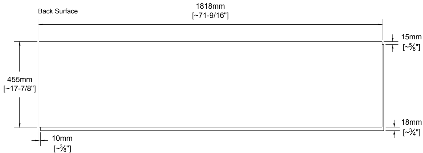
VINTAGE BRICK PANEL DETAIL SCALE: 1" = 1'-0"
