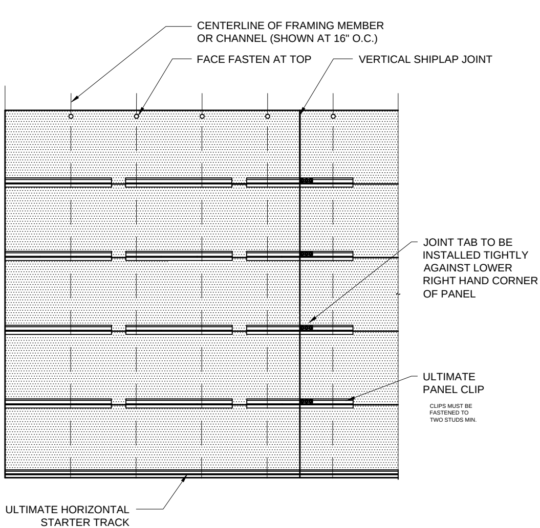
NICHIHA - CLIP PLACEMENT - STACKED PANEL LAYOUT SCALE: 1/2" = 1'-0"
