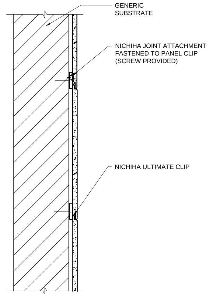
CLIP SECTION VIEW SCALE: 1-1/2" = 1'-0"
