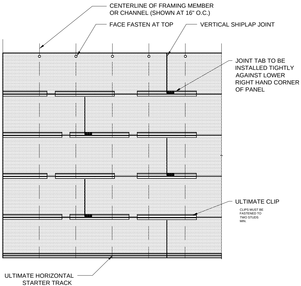
NICHIHA - CLIP PLACEMENT - STAGGERED PANEL LAYOUT - AWP1818 ONLY SCALE: 1/2" = 1'-0"
