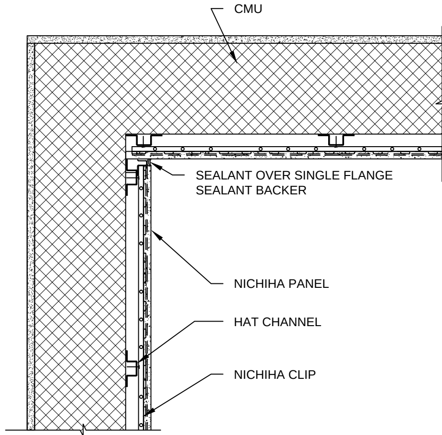
NICHIIA - AWP HORIZONTAL - CMU WITH FURRING - INSIDE CORNER
