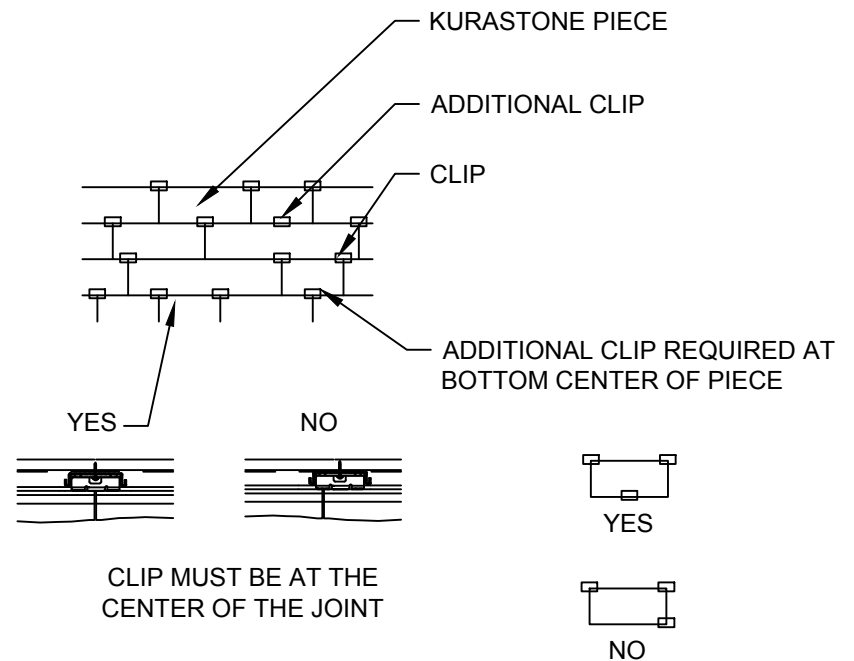
CLIP LOCATION DIAGRAM: NTS
