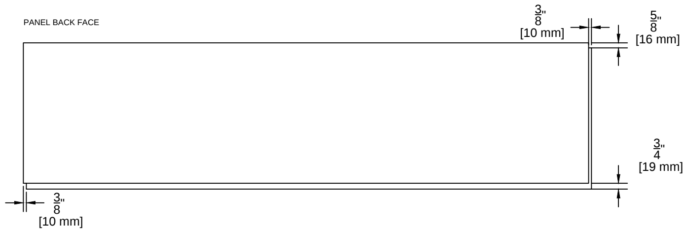
NOVENARY TILE PANEL DETAIL SCALE: 1" = 1'-0"
