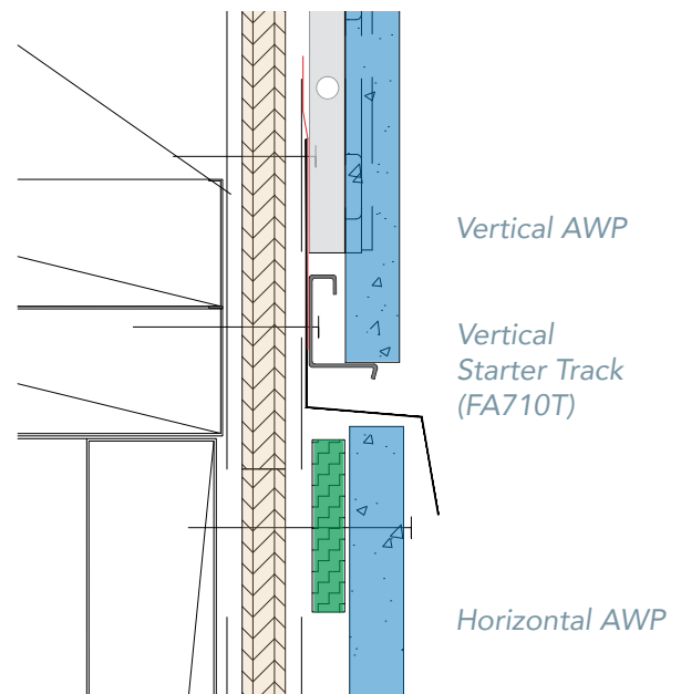
Horizontal transition joint: Compression Joint details
