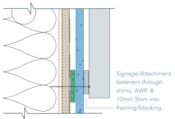
Signage/Attachments detail
