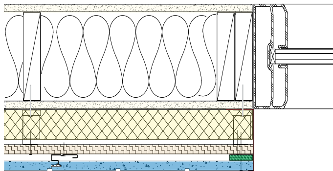
Recessed window jamb: J-profile brake metal with a min. 10mm panel face return flange. C.I. assembly shown includes thermally-broken vertical furring with min. 7/16" OSB or plywood.
