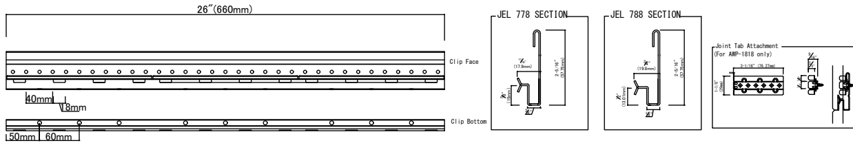
A 4 AWP CLIPS: JEL778 & JEL788 NOT-TO-SCALE
