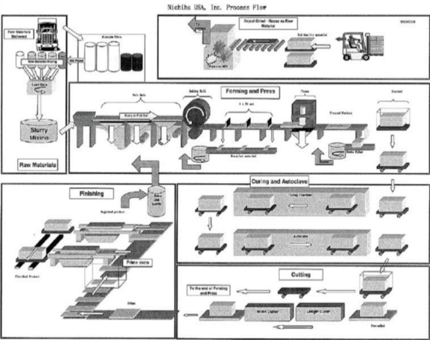
FIGURE 1. MANUFACTURING PROCESS
